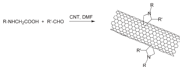
Scheme 1 General scheme for the 1,3-dipolar cycloaddition of azomethine ylides to CNTs.
