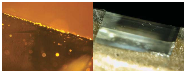
Fig. 5 Ultramicrotome knives: images of the glass (left), and diamond tool (right) taken with an optical microscope.
