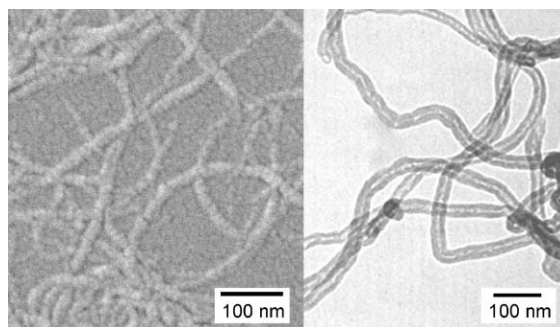
Fig. 3 Scanning electron microscopy (left) and transmission electron microscopy (right) photographs of water-soluble f -MWCNTs 1 .
