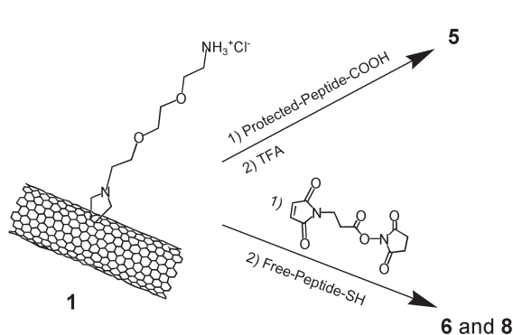
Scheme 2 Synthesis of peptide-CNT conjugates using fragment condensation ( f -CNTs 5 ) and selective chemical ligation ( f -CNTs 6 and 8 ).
