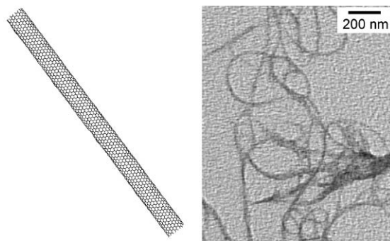
Fig. 1 Model structure of a SWCNT segment (left) and TEM image of SWCNTs (right).
