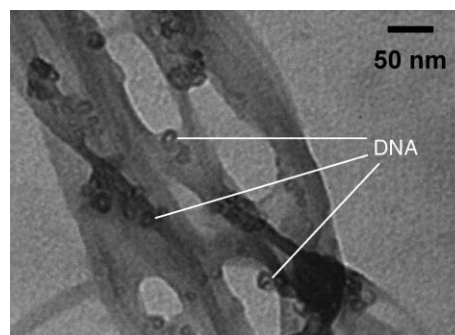
Fig. 7 TEM image f -CNTs 1 : DNA complexes.
